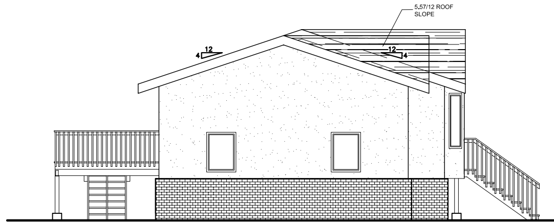
B LEFT ELEVATION A.3 SCALE : TO FIT
